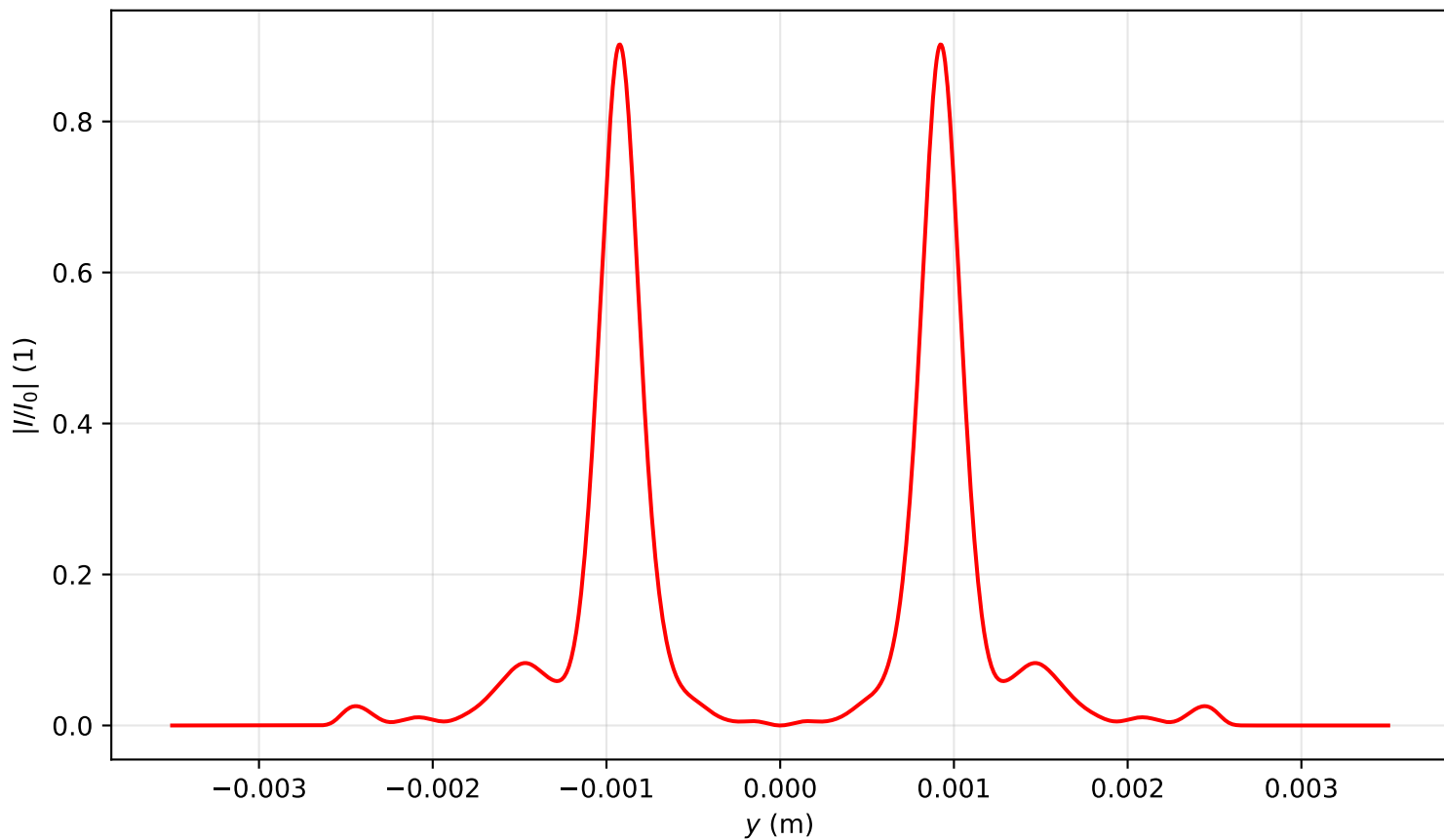
Intensity profile I(x=0, y, z=3.184)/I_0 , P_{in}=15.0\text{Pcr} , artificial time
