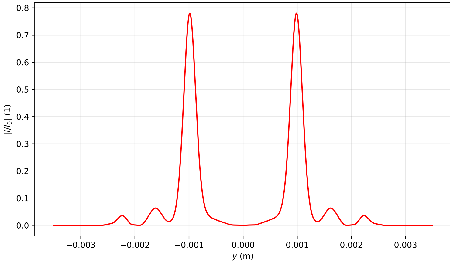
Intensity profile I(x=0, y, z=3.423)/I_0 , P_{in}=15.0P_{cr} , artificial time
