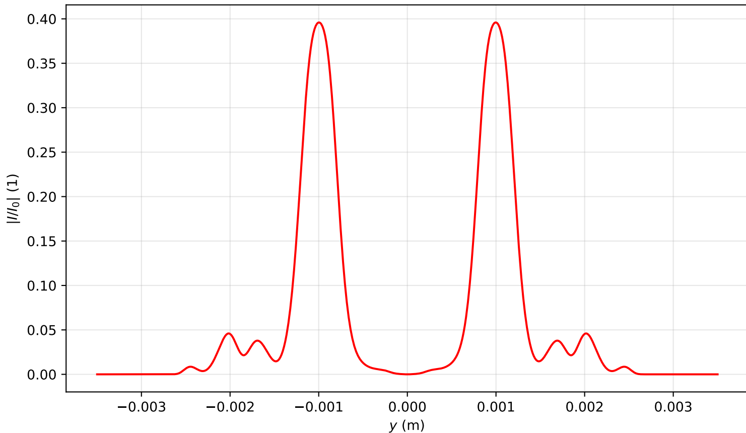
Intensity profile I(x=0, y, z=3.742)/I_0 , P_{in}=15.0P_{cr} , artificial time
