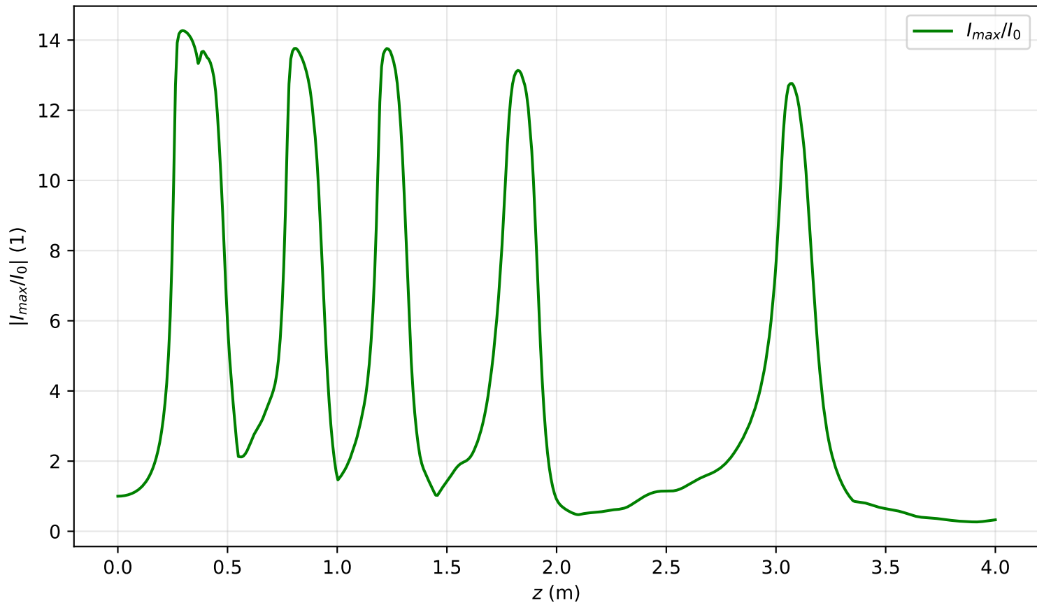
I_{\max}(x=0, y=0, z)/I_0 , \text{Pin}=16.0\text{Pcr} , artificial time
