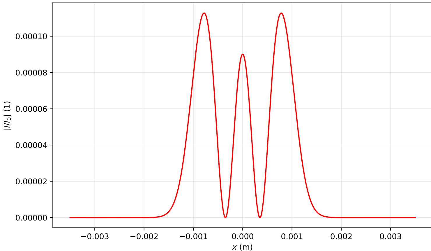
Intensity profile I(x, y = 0, z = 0.080)/I_0 , P_{in}=16.0P_{cr} , artificial time
