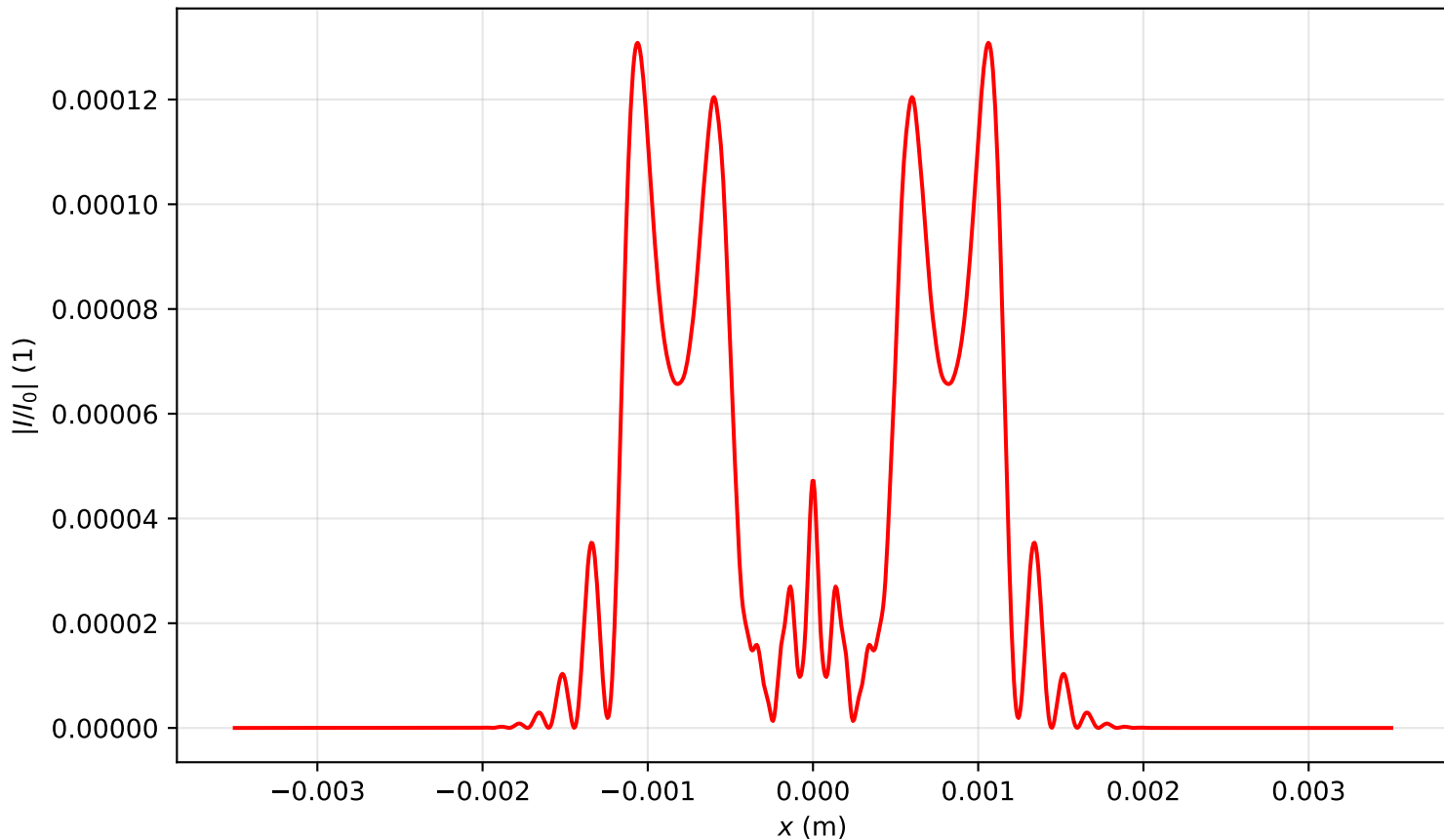
Intensity profile I(x, y = 0, z = 0.398)/I_0 , P_{in}=16.0P_{cr} , artificial time
