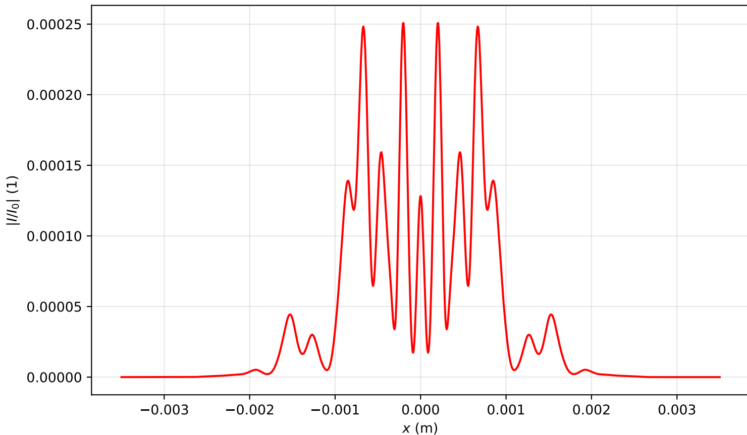
Intensity profile I(x, y = 0, z = 0.637)/I_0 , P_{in}=16.0P_{cr} , artificial time
