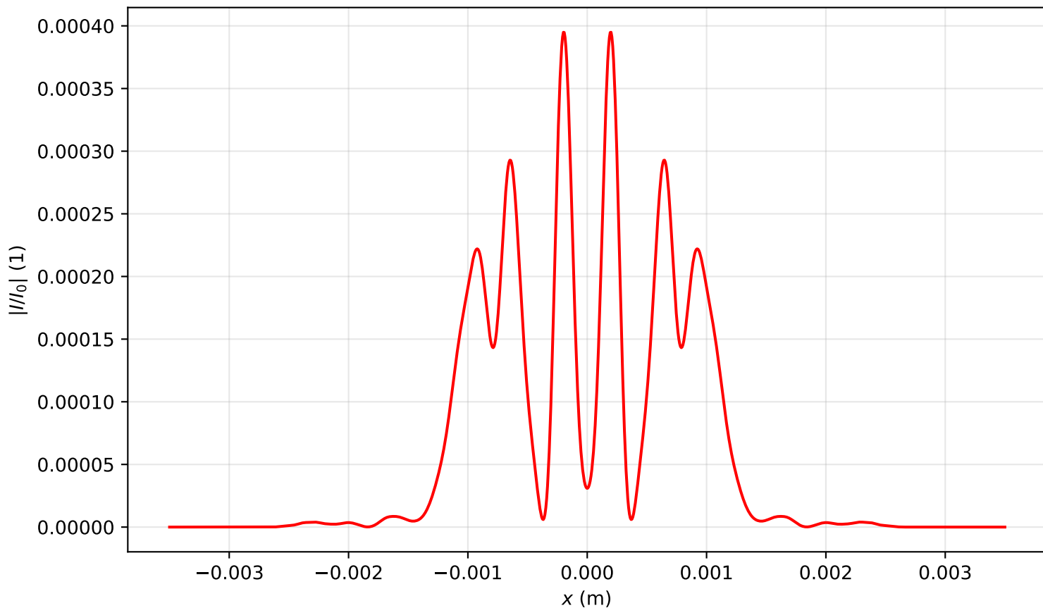
Intensity profile I(x, y = 0, z = 0.876)/I_0 , P_{in}=16.0P_{cr} , artificial time
