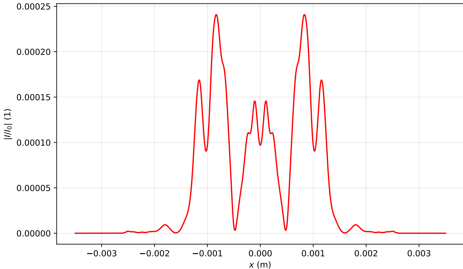
Intensity profile I(x, y = 0, z = 1.035)/I_0 , P_{in}=16.0P_{cr} , artificial time
