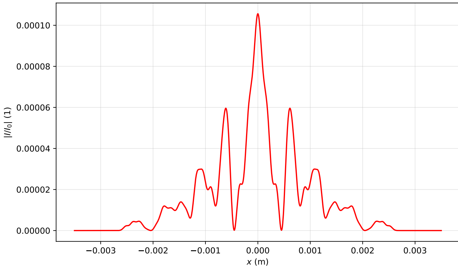
Intensity profile I(x, y = 0, z = 1.194)/I_0 , P_{in}=16.0P_{cr} , artificial time
