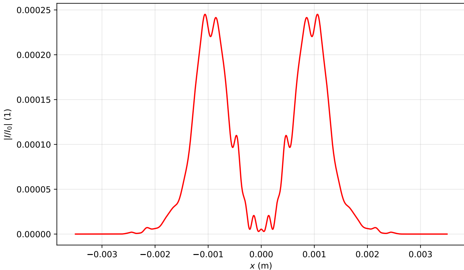
Intensity profile I(x, y = 0, z = 1.672)/I_0 , P_{in}=16.0P_{cr} , artificial time
