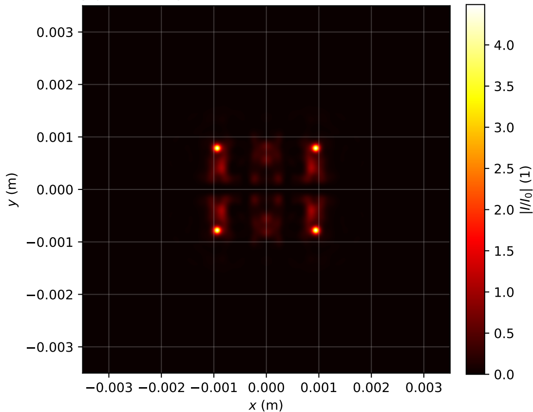
Intensity profile I(x, y, z = 0.955)/I_0 , P_{in}=16.0\text{Pcr} , artificial time
