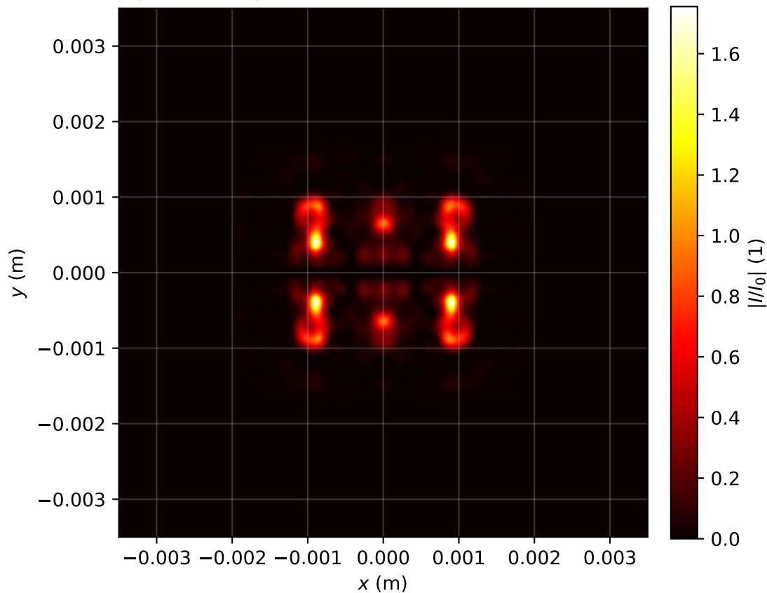
Intensity profile I(x, y, z = 1.035)/I_0 , P_{in}=16.0\text{Pcr} , artificial time
