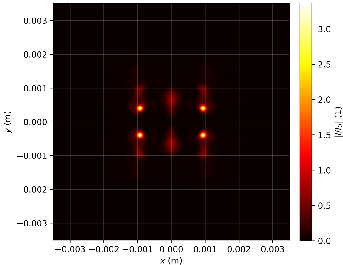
Intensity profile I(x, y, z = 1.353)/I_0 , P_{in}=16.0\text{Pcr} , artificial time
