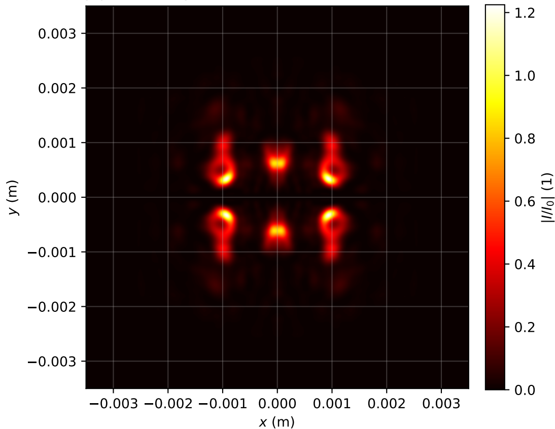
Intensity profile I(x, y, z = 1.433)/I_0 , P_{in}=16.0\text{Pcr} , artificial time
