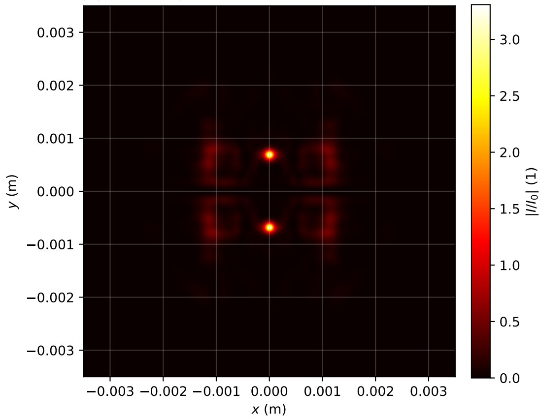
Intensity profile I(x, y, z = 1.672)/I_0 , P_{in}=16.0\text{Pcr} , artificial time
