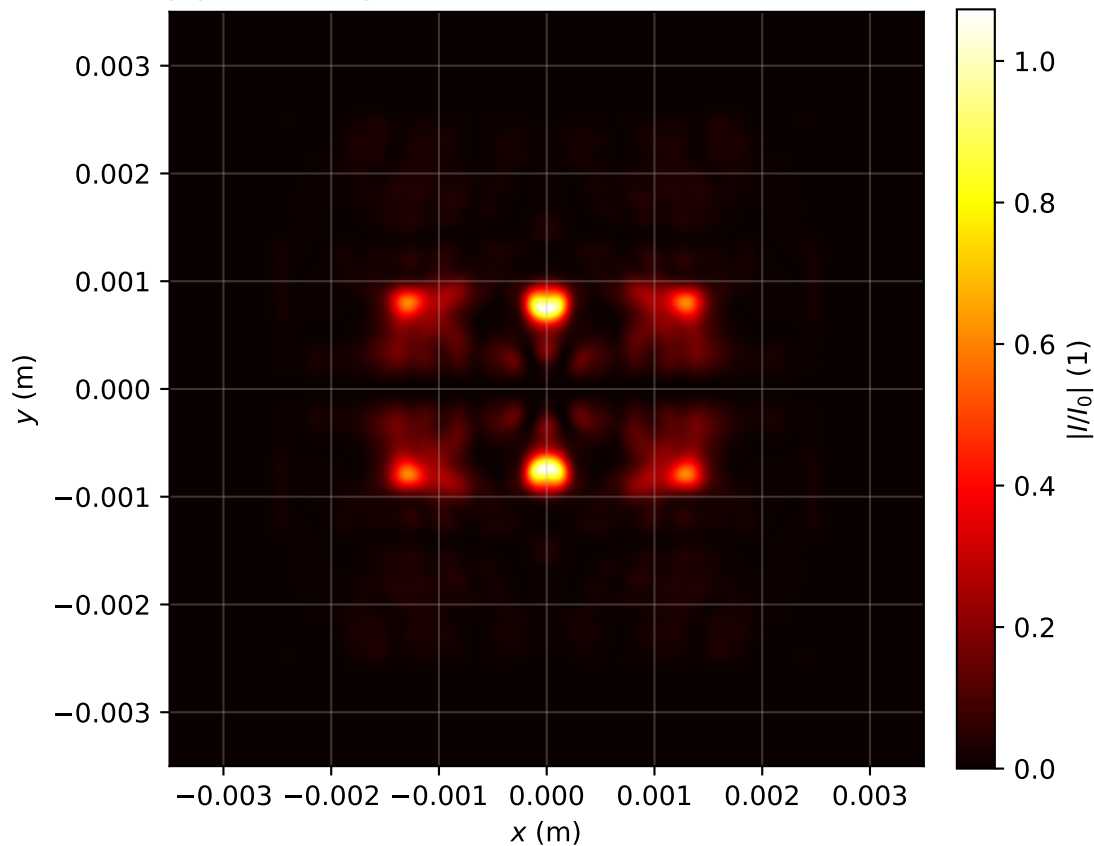
Intensity profile I(x, y, z = 1.990)/I_0 , P_{in}=16.0\text{Pcr} , artificial time
