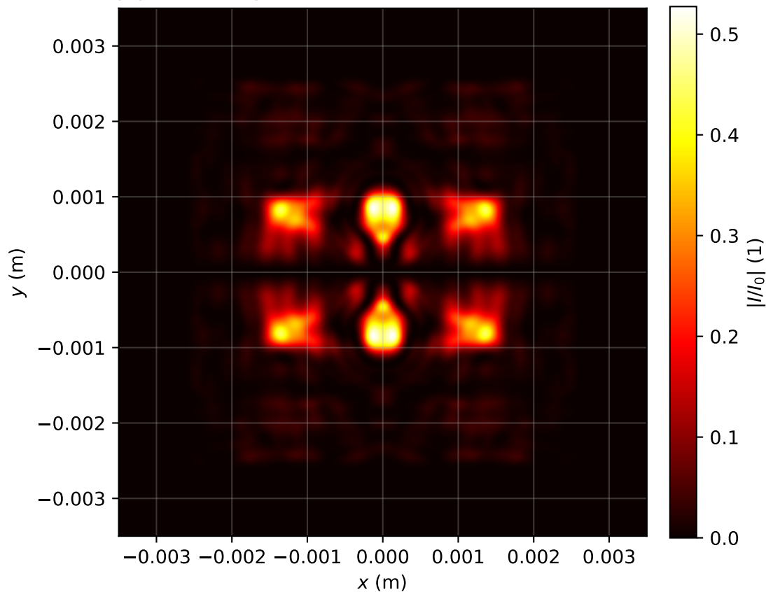
Intensity profile I(x, y, z = 2.070)/I_0 , P_{in}=16.0P_{cr} , artificial time
