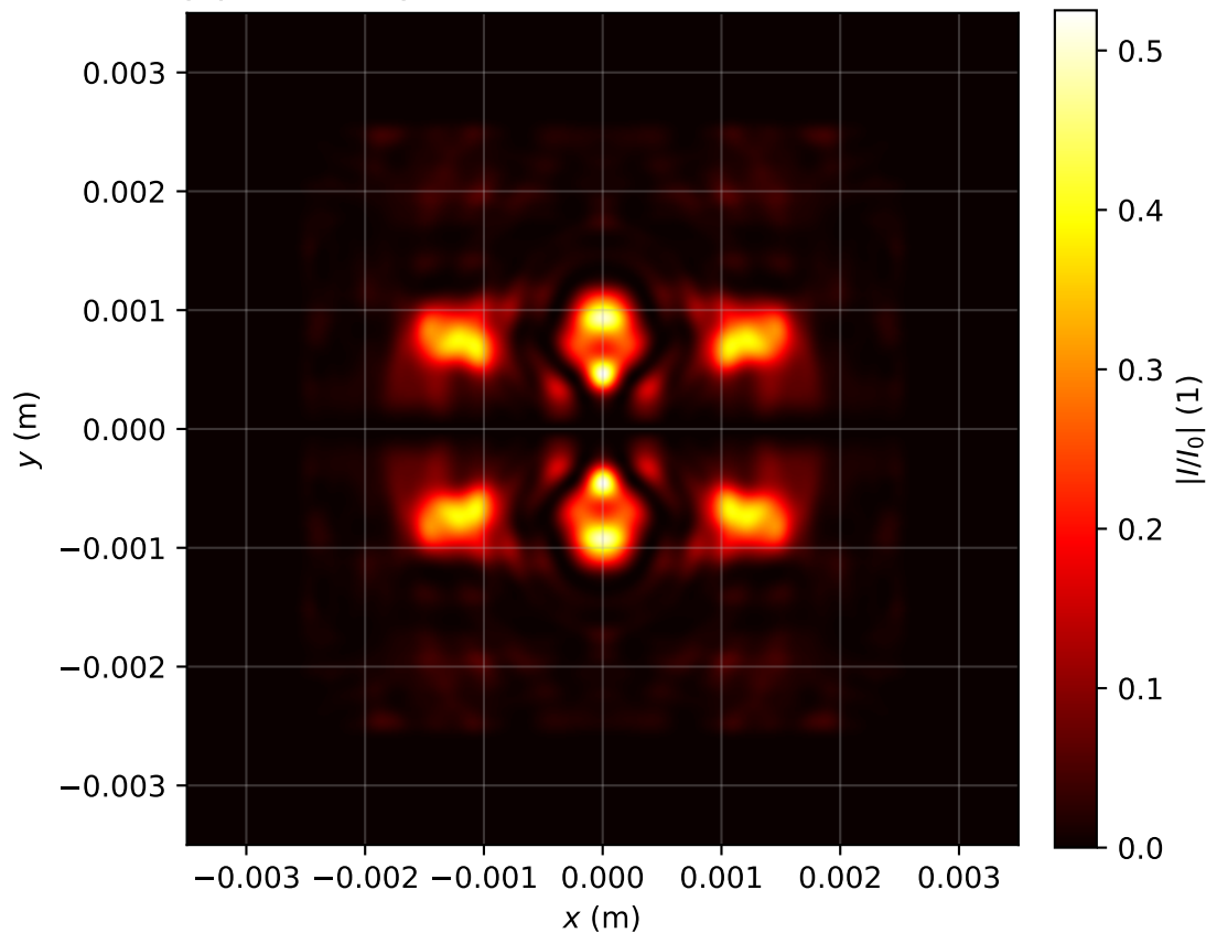
Intensity profile I(x, y, z = 2.149)/I_0 , P_{in}=16.0\text{Pcr} , artificial time
