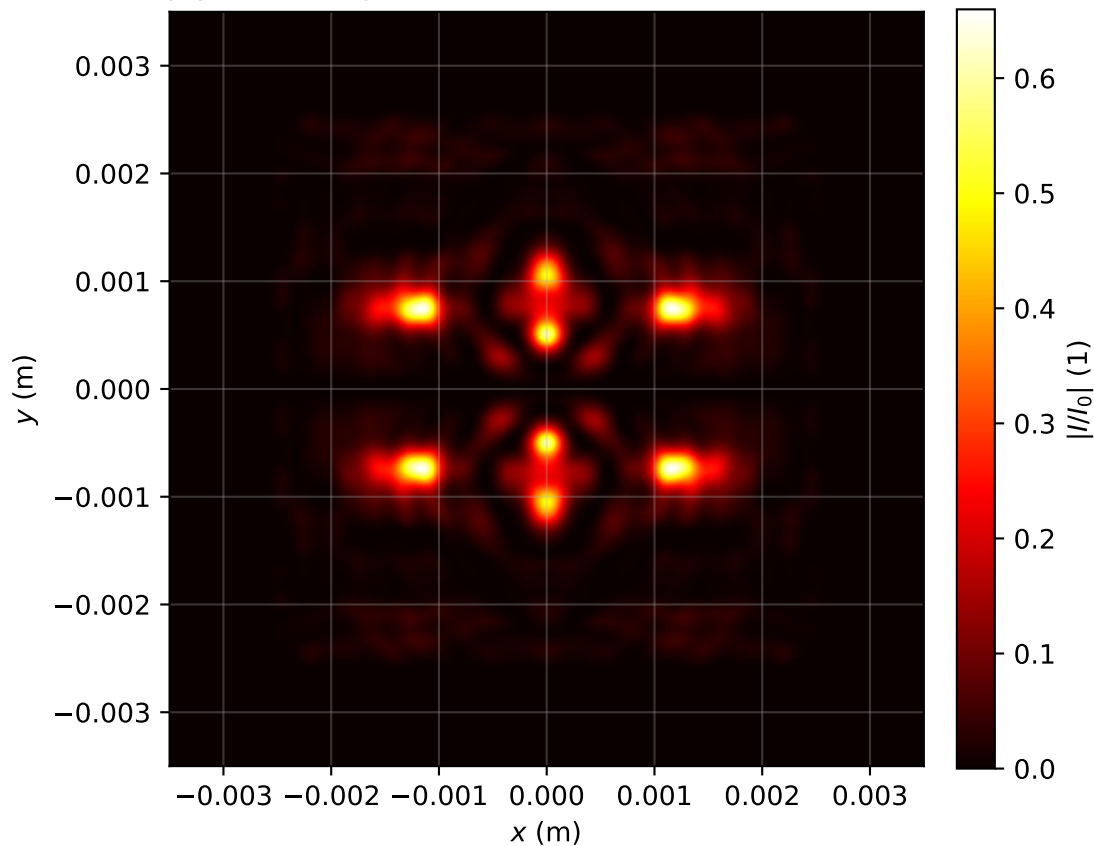
Intensity profile I(x, y, z = 2.309)/I_0 , P_{in}=16.0P_{cr} , artificial time
