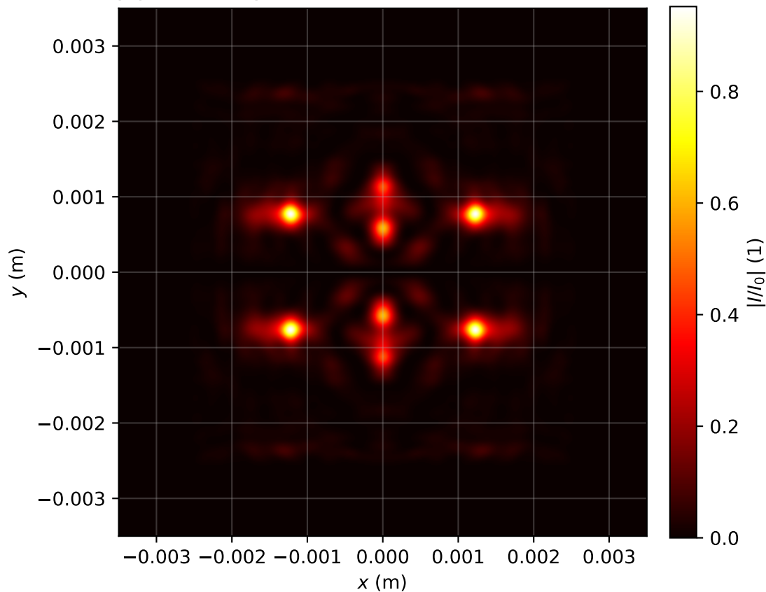
Intensity profile I(x, y, z = 2.388)/I_0 , P_{in}=16.0\text{Pcr} , artificial time
