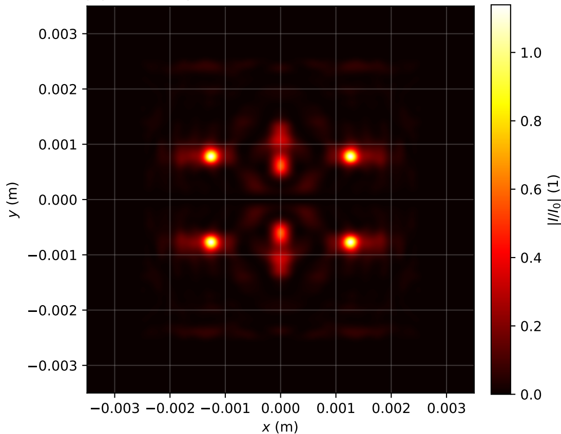
Intensity profile I(x, y, z = 2.468)/I_0 , P_{in}=16.0\text{Pcr} , artificial time
