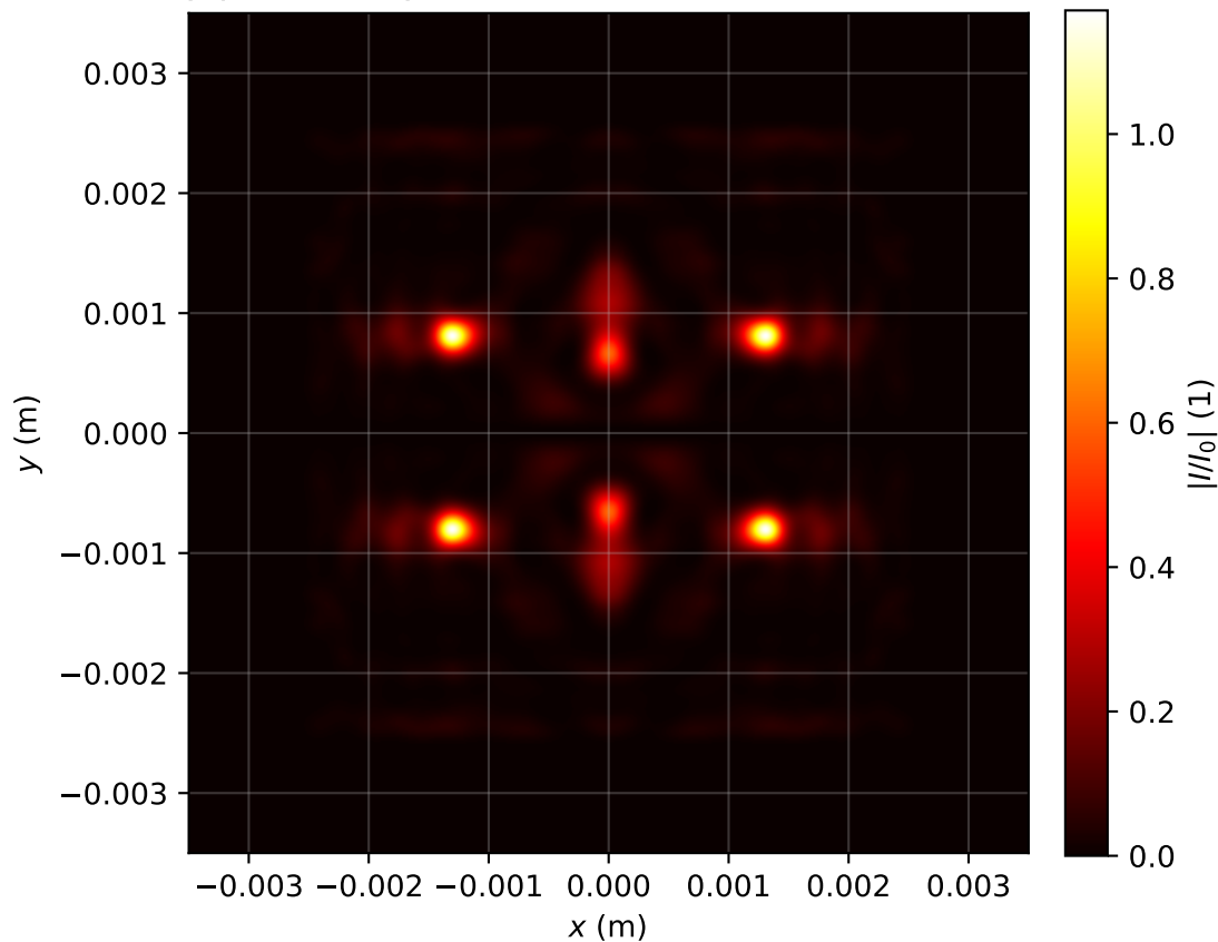
Intensity profile I(x, y, z = 2.548)/I_0 , P_{in}=16.0\text{Pcr} , artificial time
