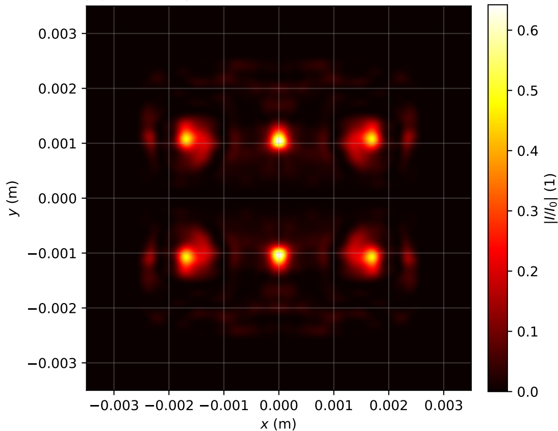
Intensity profile I(x, y, z = 3.503)/I_0 , P_{in}=16.0\text{Pcr} , artificial time
