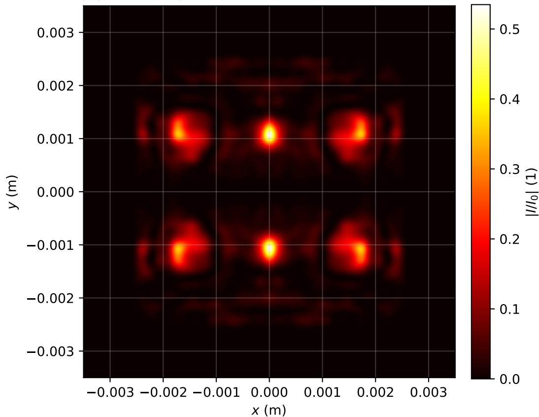
Intensity profile I(x, y, z = 3.582)/I_0 , P_{in}=16.0P_{cr} , artificial time
