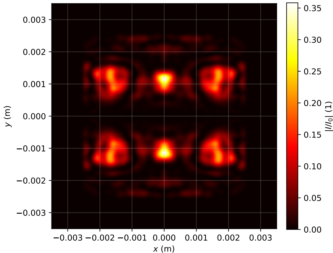
Intensity profile I(x, y, z = 3.742)/I_0 , P_{in}=16.0P_{cr} , artificial time
