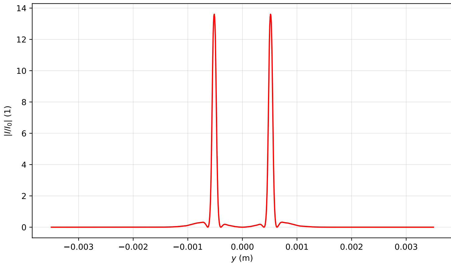
Intensity profile I(x=0, y, z=0.398)/I_0 , \text{Pin}=16.0\text{Pcr} , artificial time
