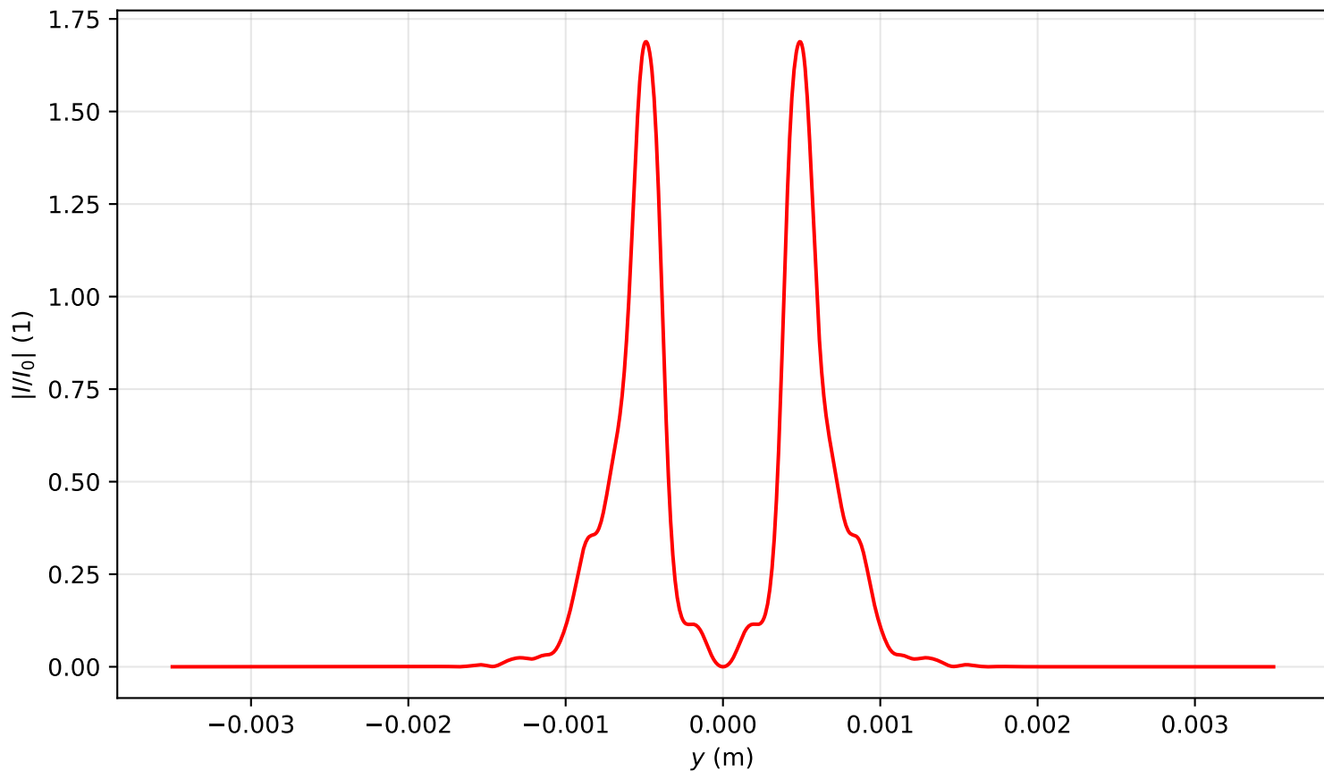
Intensity profile I(x = 0, y, z = 0.557)/I_0 , P_{in}=16.0P_{cr} , artificial time
