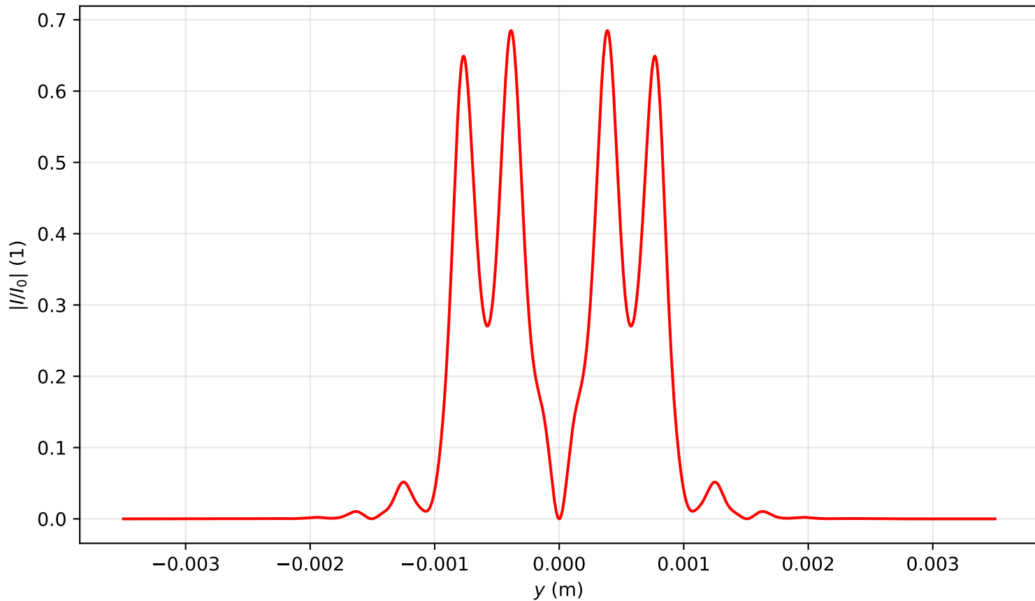
Intensity profile I(x=0, y, z=0.716)/I_0 , P_{in}=16.0P_{cr} , artificial time
