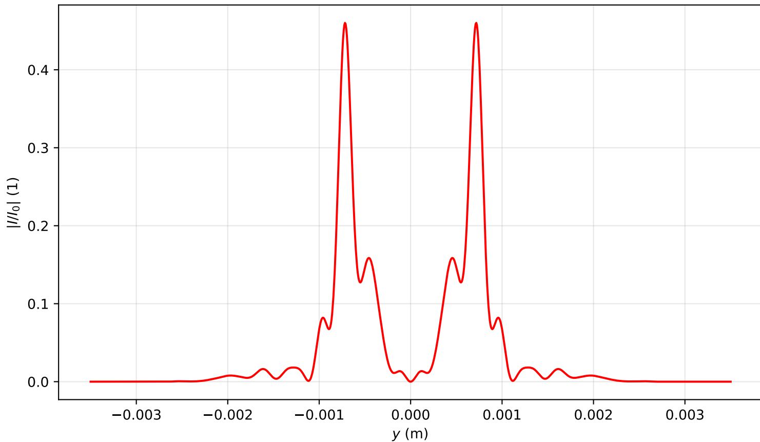
Intensity profile I(x=0, y, z=0.876)/I_0 , P_{in}=16.0P_{cr} , artificial time
