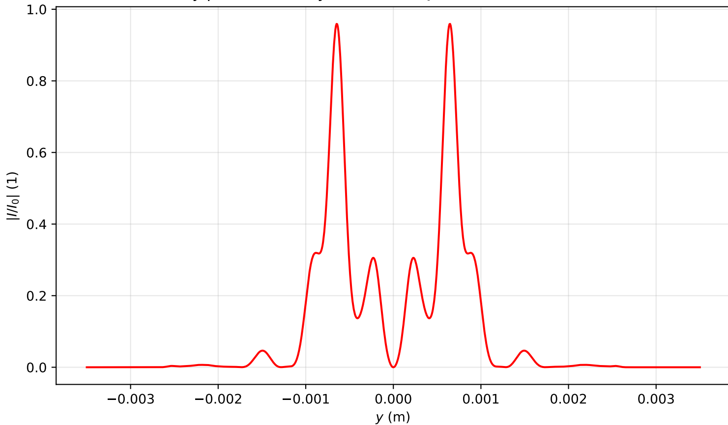
Intensity profile I(x=0, y, z=1.035)/I_0 , P_{in}=16.0\text{Pcr} , artificial time
