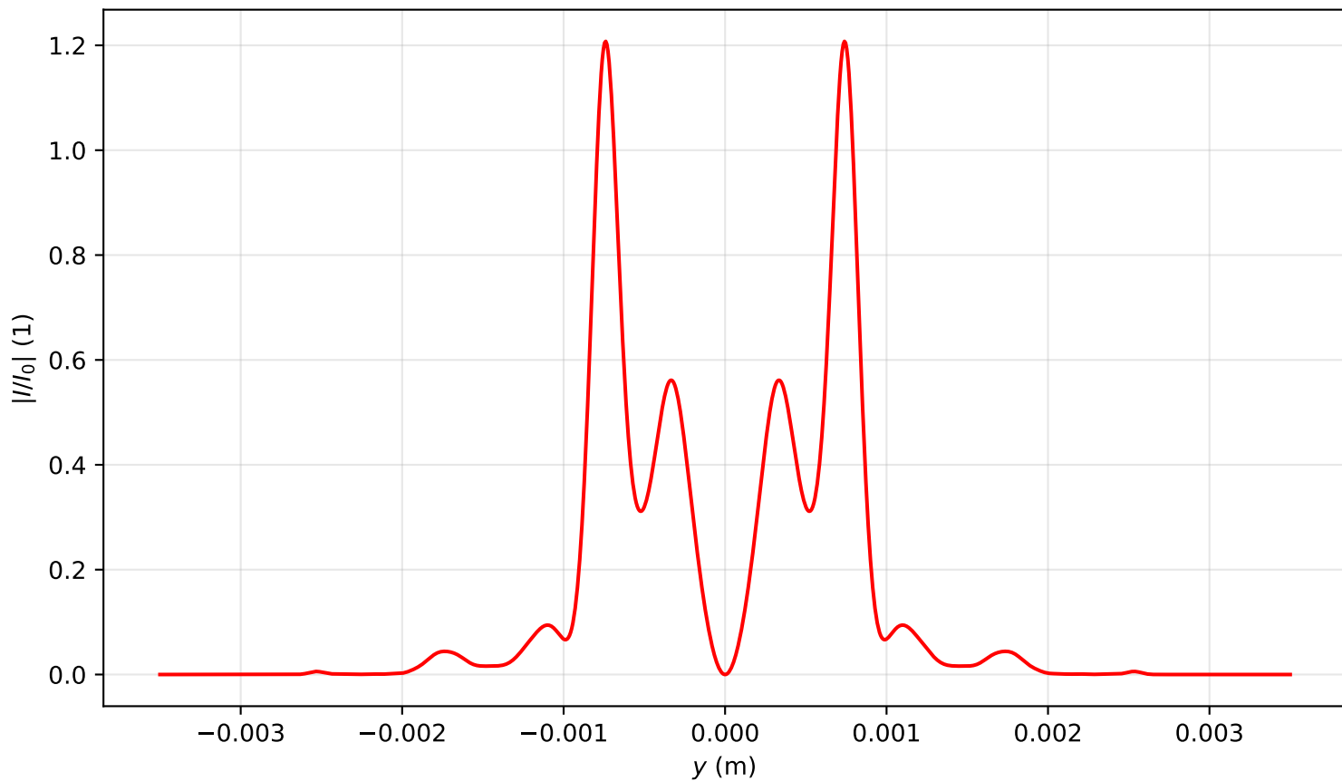
Intensity profile I(x=0, y, z=1.194)/I_0 , P_{in}=16.0P_{cr} , artificial time
