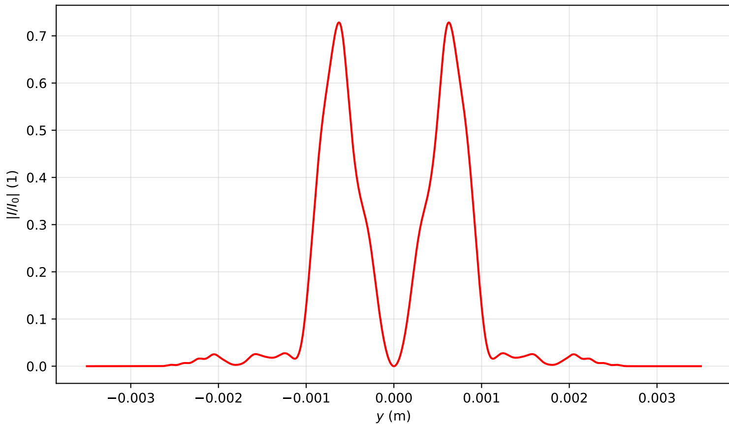
Intensity profile I(x=0, y, z=1.353)/I_0 , P_{in}=16.0P_{cr} , artificial time
