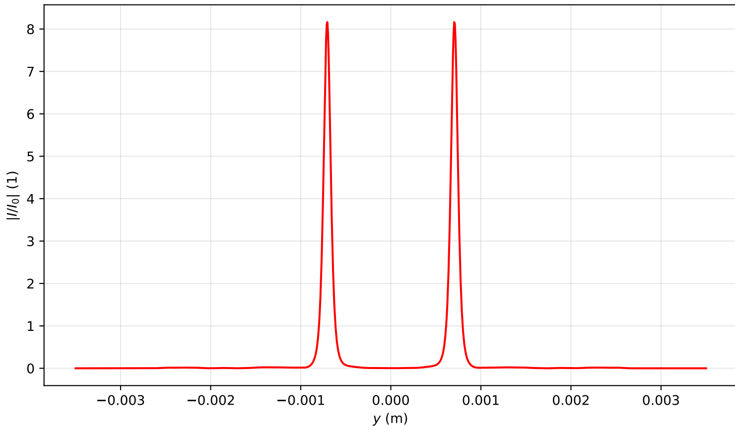
Intensity profile I(x=0, y, z=1.751)/I_0 , P_{in}=16.0\text{Pcr} , artificial time
