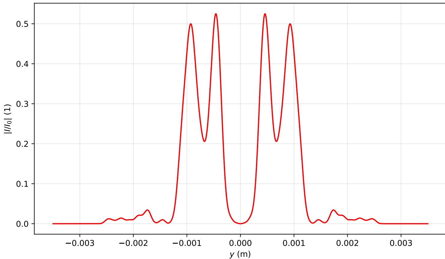
Intensity profile I(x=0, y, z=2.149)/I_0 , P_{in}=16.0P_{cr} , artificial time
