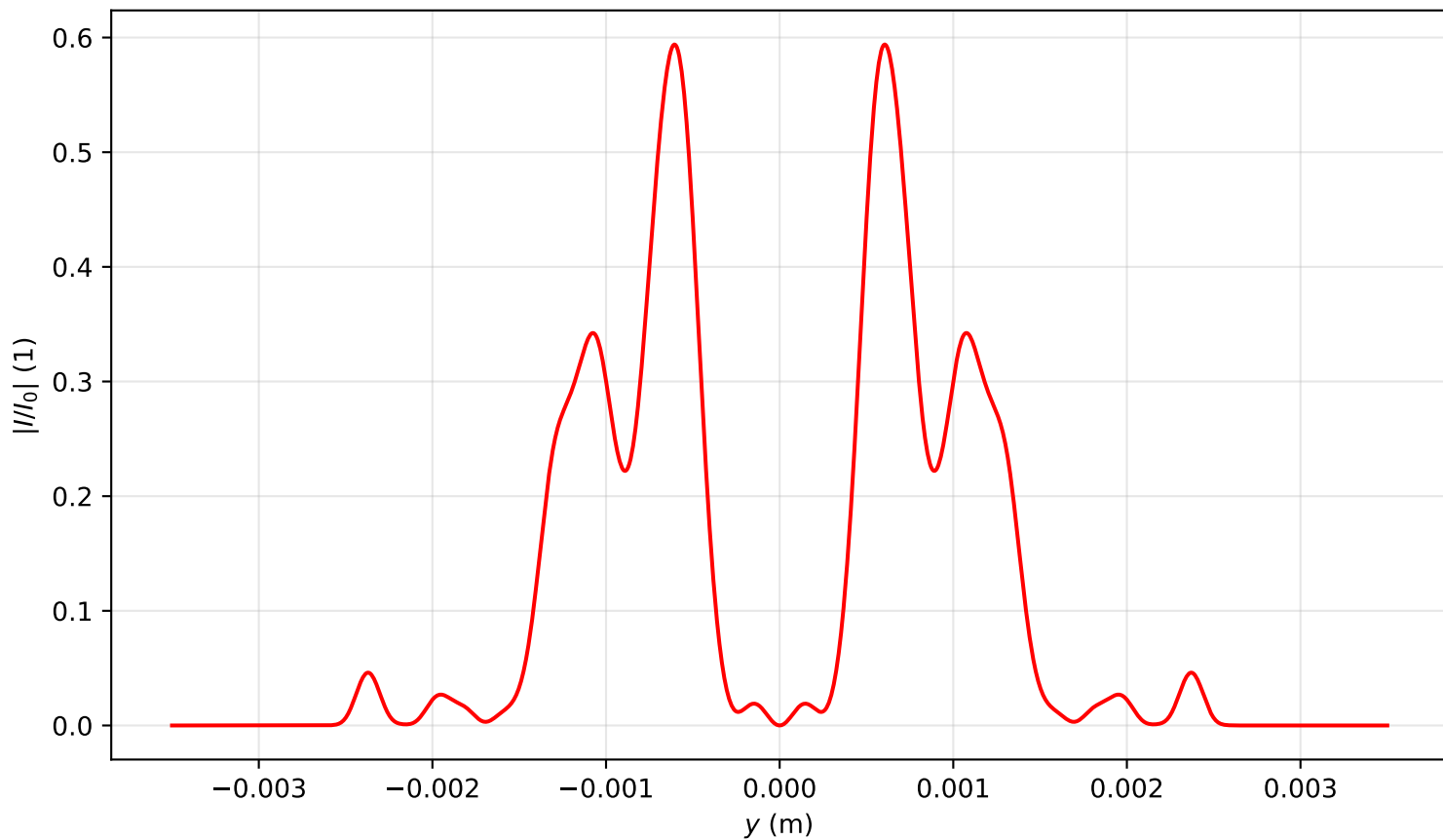
Intensity profile I(x=0, y, z=2.468)/I_0 , P_{in}=16.0P_{cr} , artificial time
