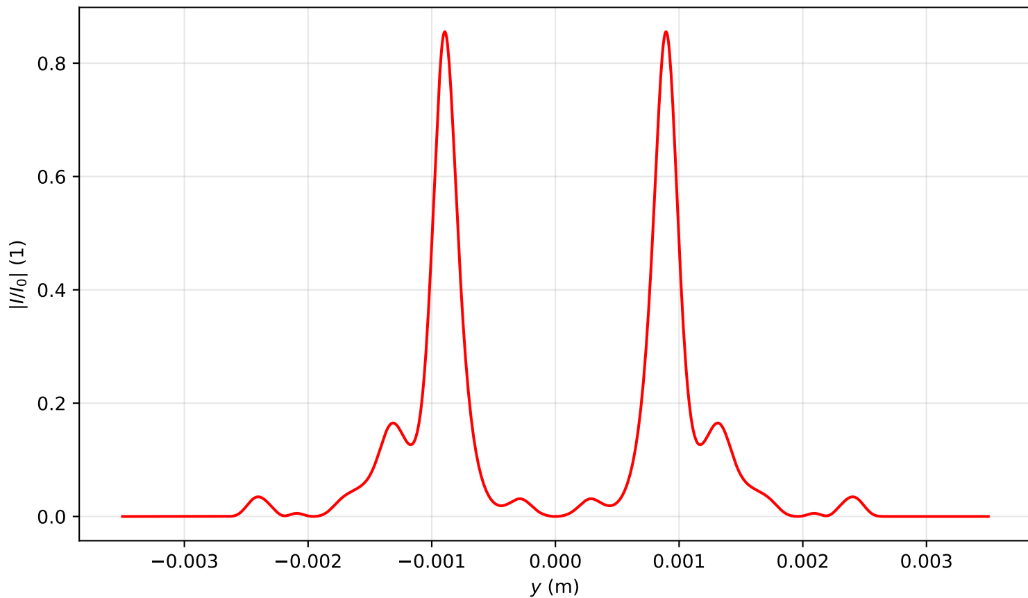
Intensity profile I(x=0, y, z=2.946)/I_0 , P_{in}=16.0P_{cr} , artificial time
