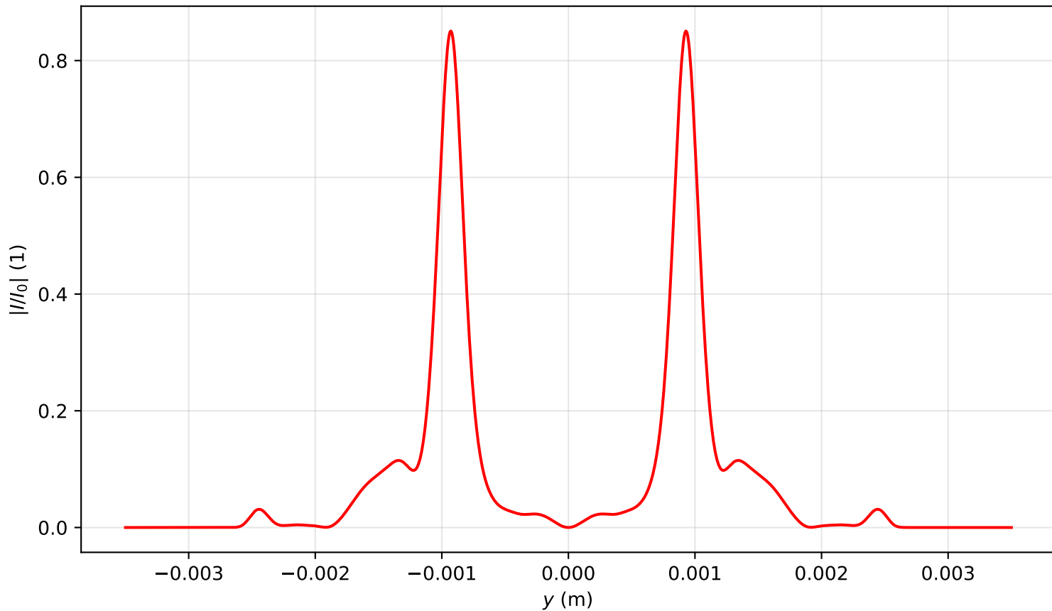
Intensity profile I(x=0, y, z=3.025)/I_0 , P_{in}=16.0P_{cr} , artificial time
