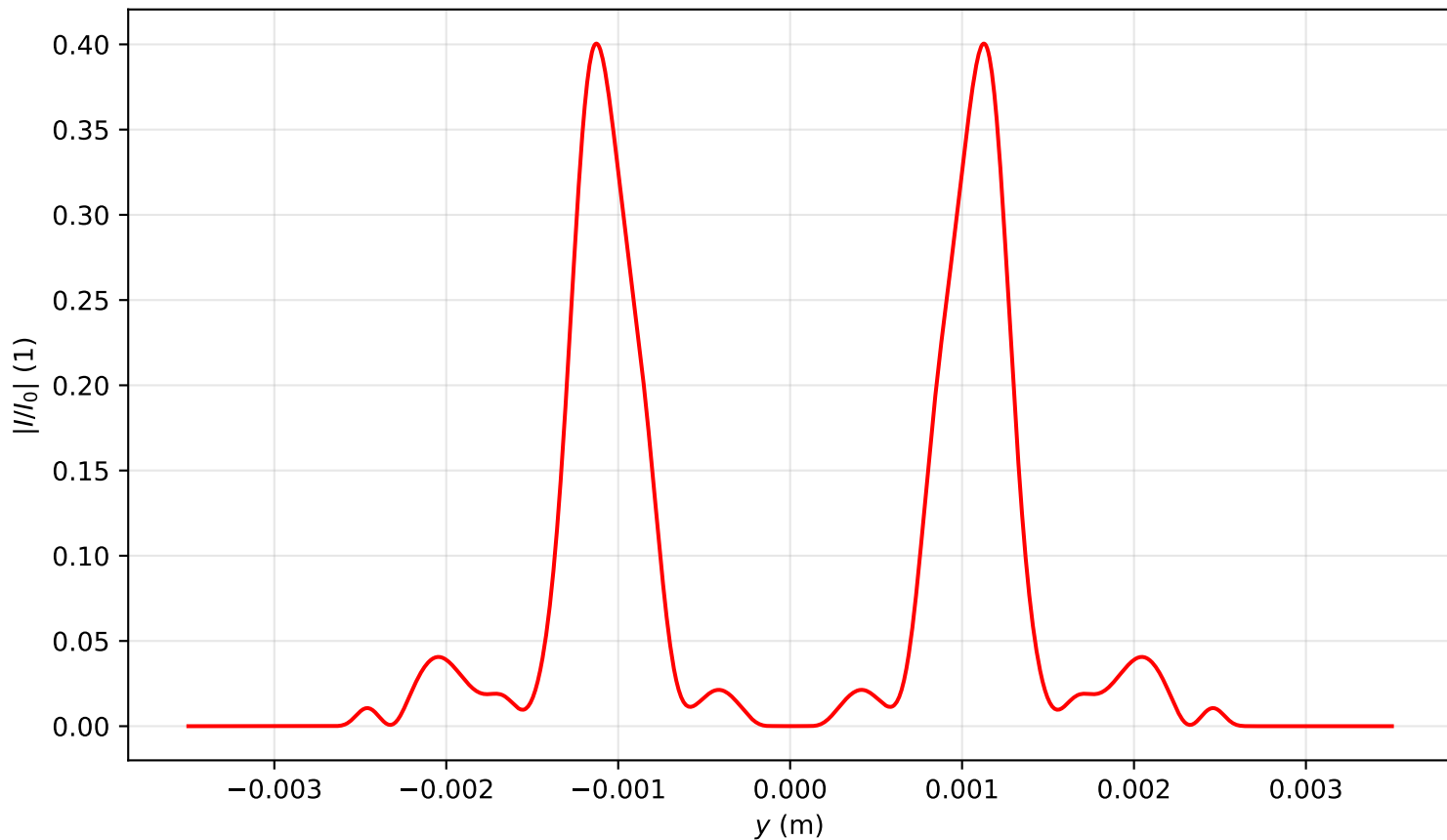
Intensity profile I(x=0, y, z=3.662)/I_0 , P_{in}=16.0P_{cr} , artificial time
