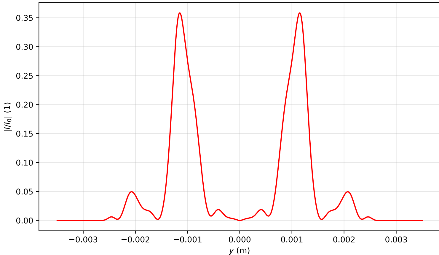
Intensity profile I(x=0, y, z=3.742)/I_0 , P_{in}=16.0\text{Pcr} , artificial time
