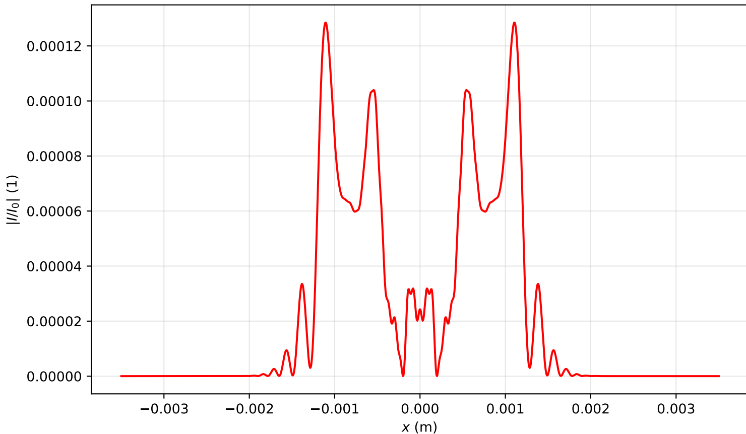
Intensity profile I(x, y = 0, z = 0.398)/I_0 , P_{in}=17.0P_{cr} , artificial time
