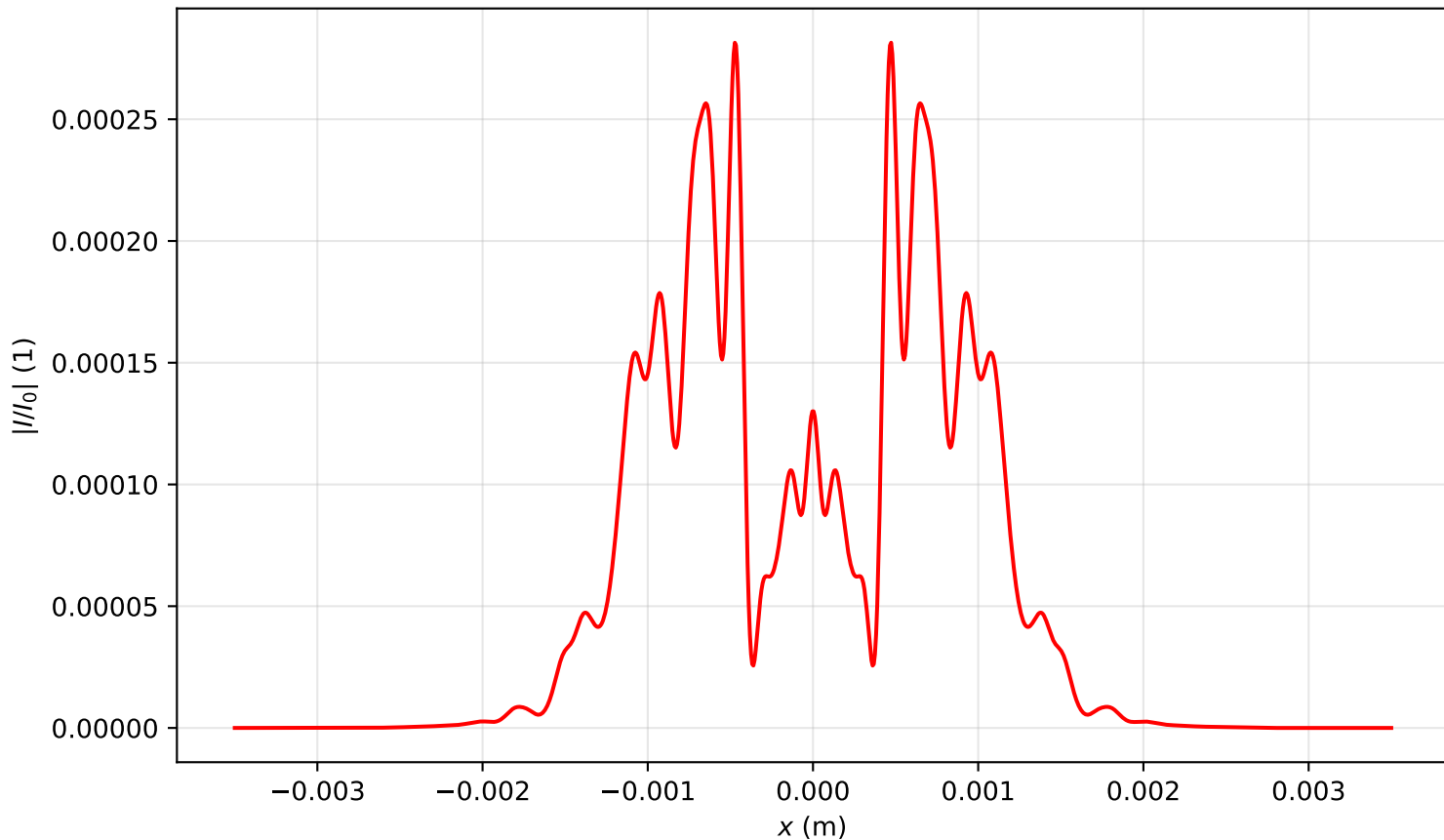
Intensity profile I(x, y = 0, z = 0.557)/I_0 , P_{in}=17.0\text{Pcr} , artificial time
