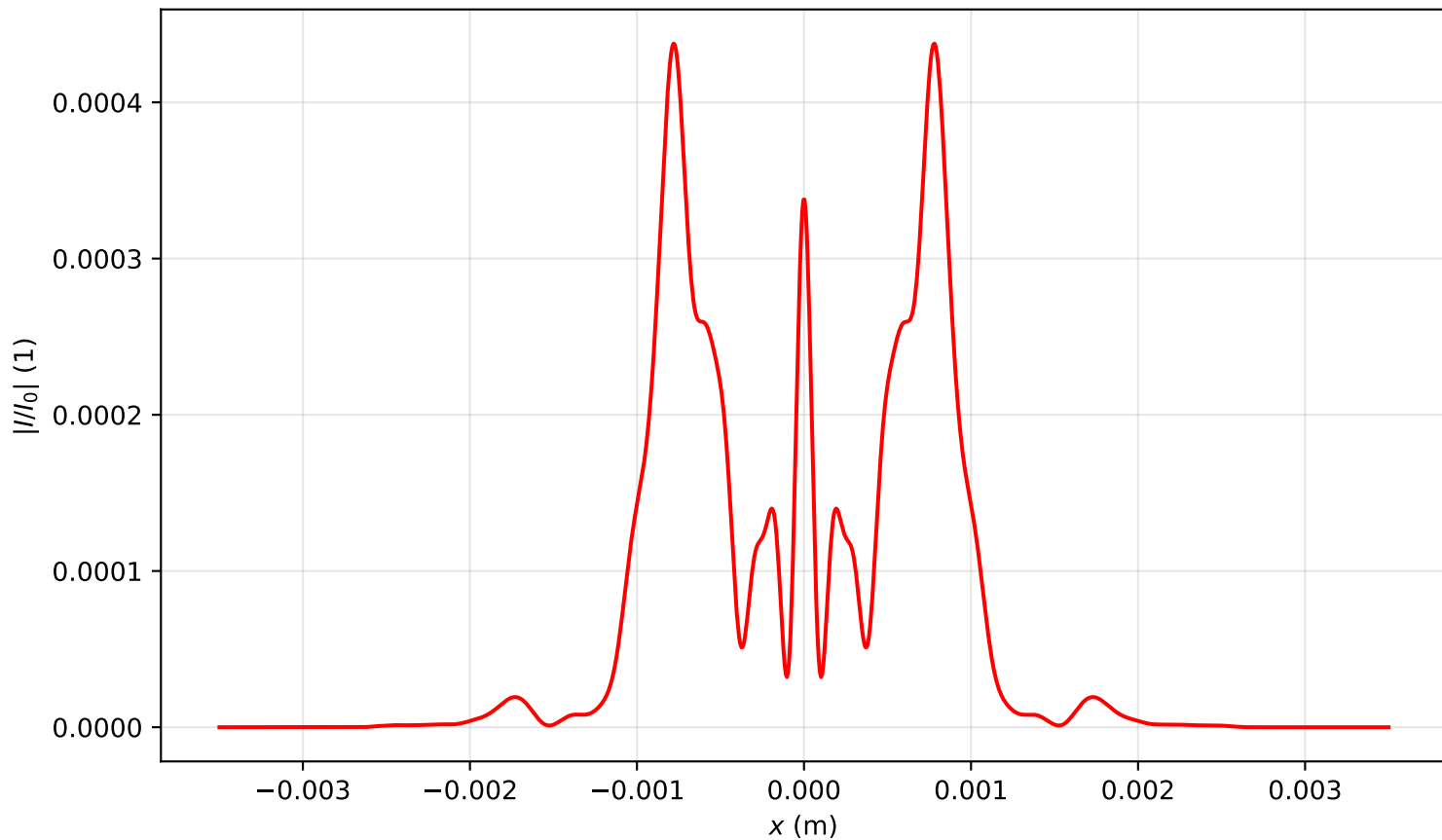
Intensity profile I(x, y = 0, z = 0.716)/I_0 , P_{in}=17.0\text{Pcr} , artificial time
