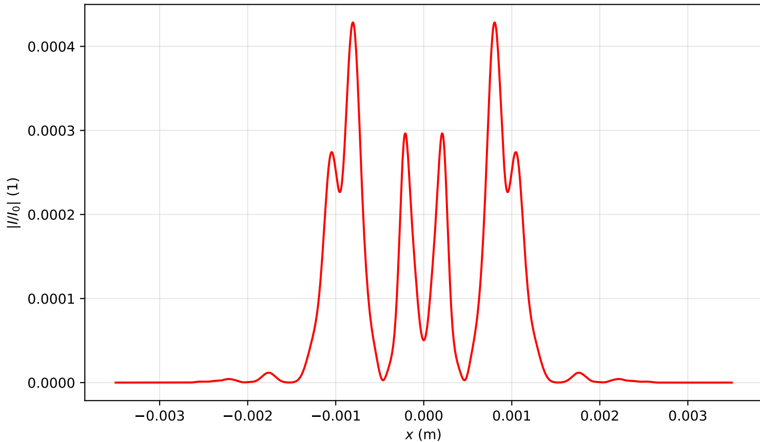
Intensity profile I(x, y = 0, z = 0.955)/I_0 , P_{in}=17.0\text{Pcr} , artificial time
