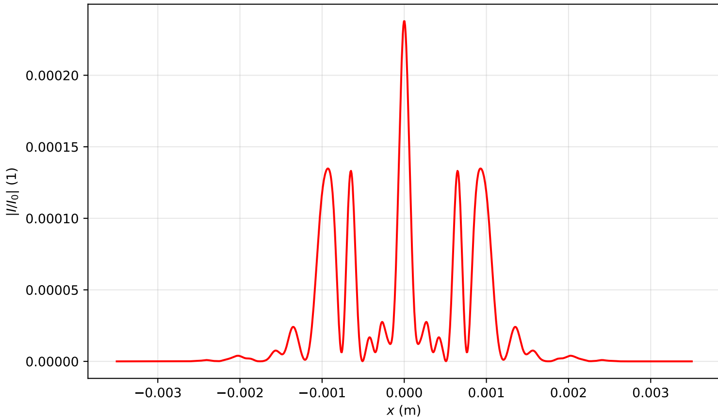
Intensity profile I(x, y = 0, z = 1.194)/I_0 , P_{in}=17.0P_{cr} , artificial time
