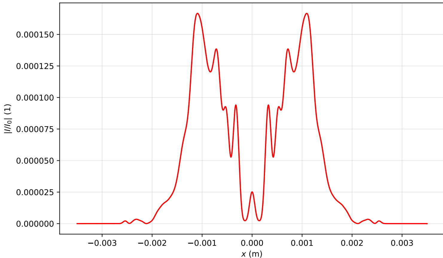
Intensity profile I(x, y = 0, z = 1.592)/I_0 , P_{in}=17.0\text{Pcr} , artificial time
