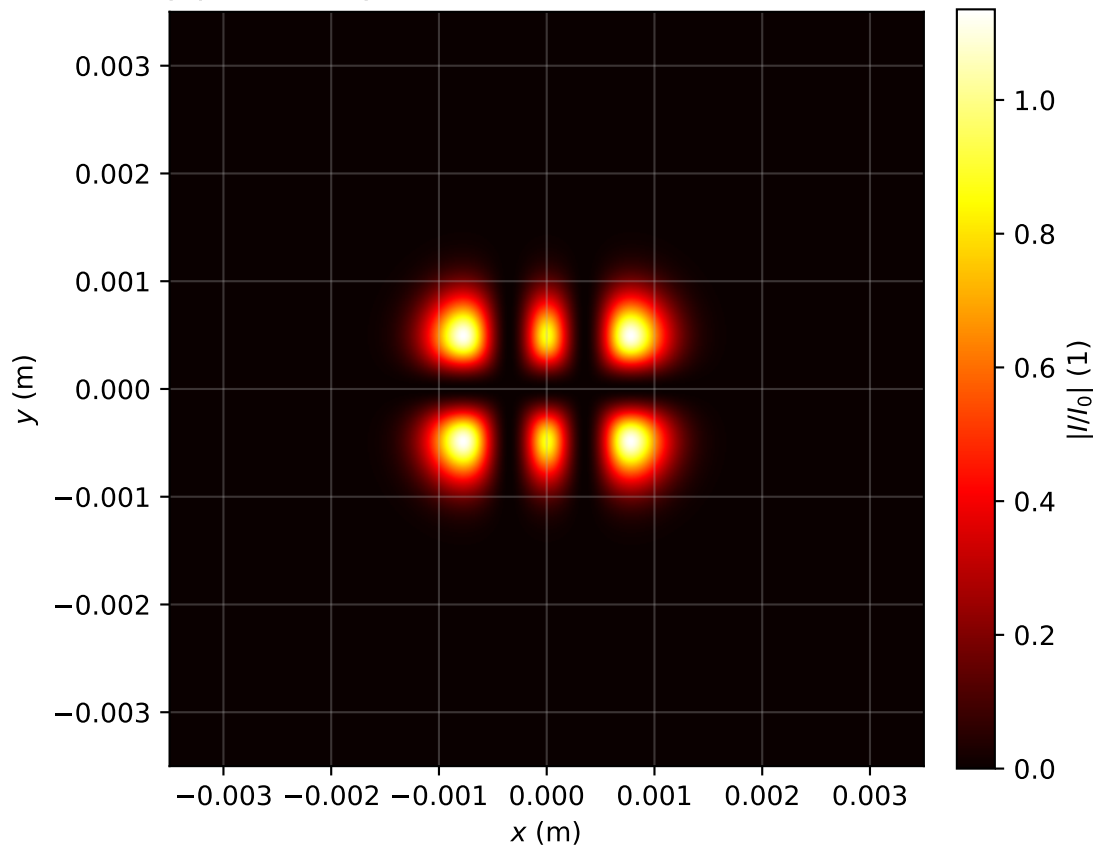
Intensity profile I(x, y, z = 0.080)/I_0 , P_{in}=17.0\text{Pcr} , artificial time
