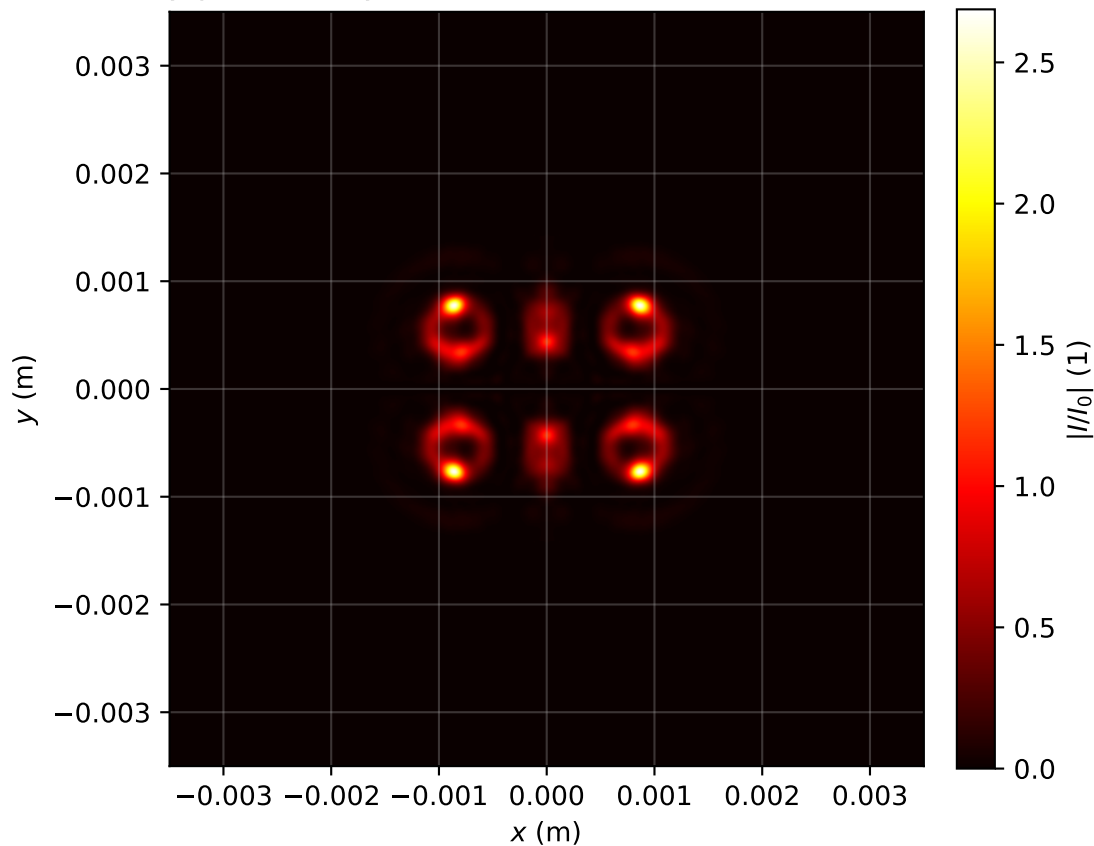
Intensity profile I(x, y, z = 0.557)/I_0 , P_{in}=17.0\text{Pcr} , artificial time
