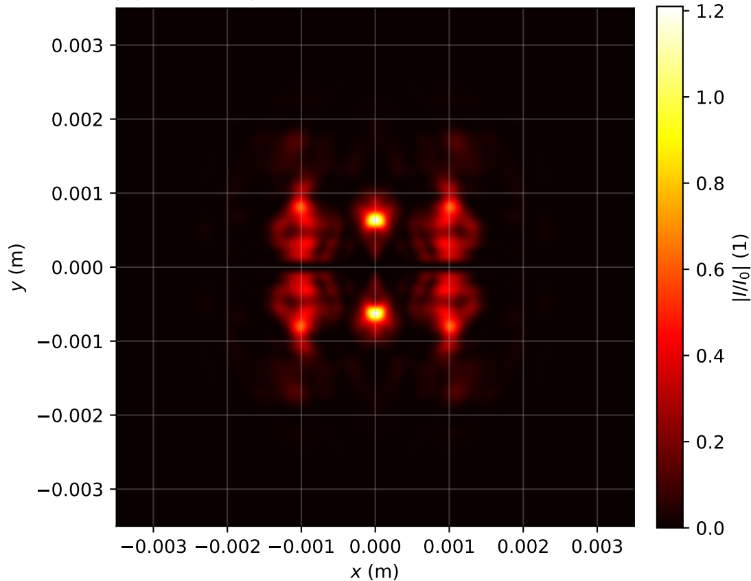
Intensity profile I(x, y, z = 1.433)/I_0 , P_{in}=17.0\text{Pcr} , artificial time
