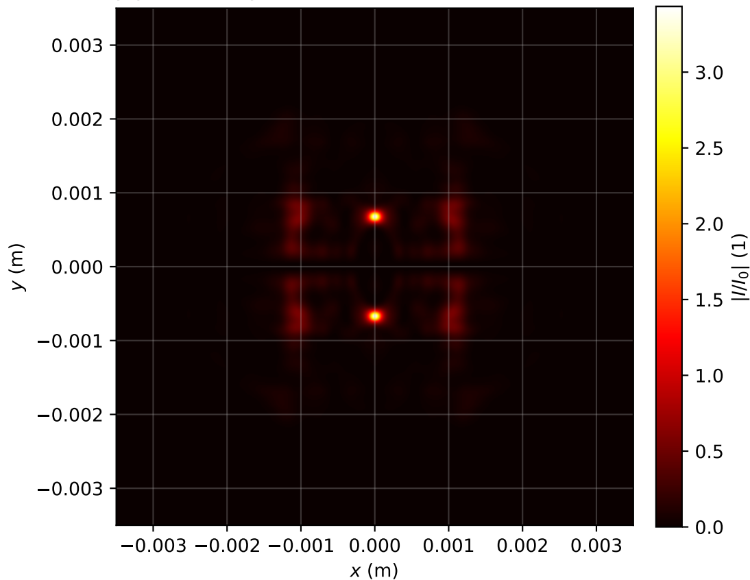
Intensity profile I(x, y, z = 1.592)/I_0 , P_{in}=17.0\text{Pcr} , artificial time
